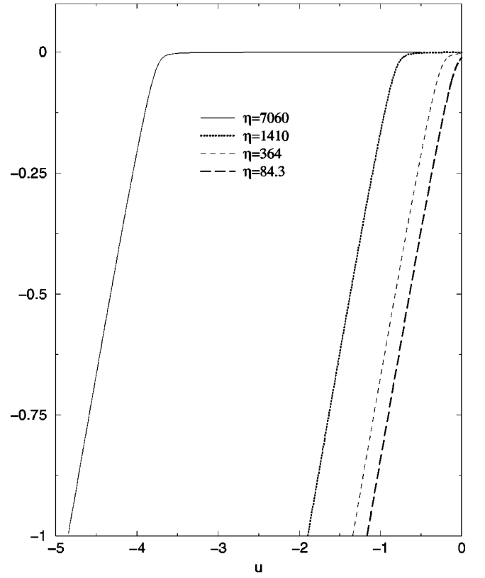
FIG. 5. \hat{\tau}(u) versus u for 4 values of \eta .
